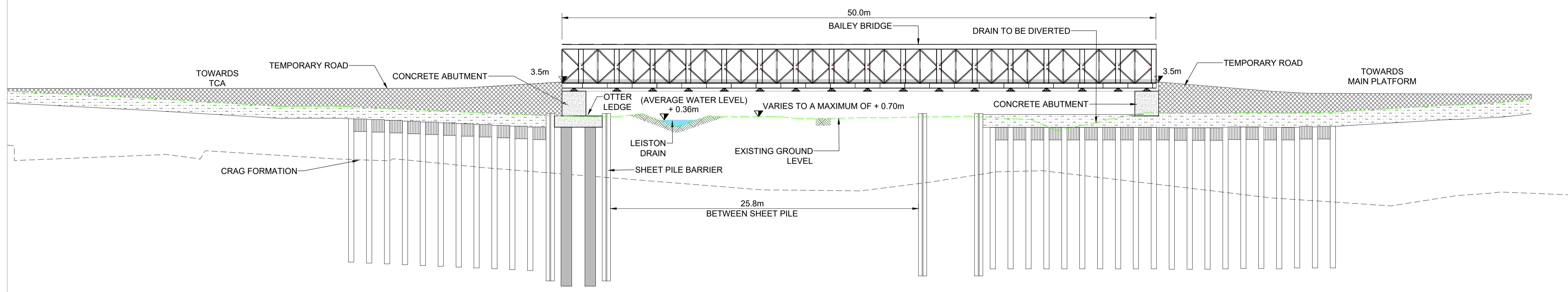
SECTION A - A SCALE 1:200
