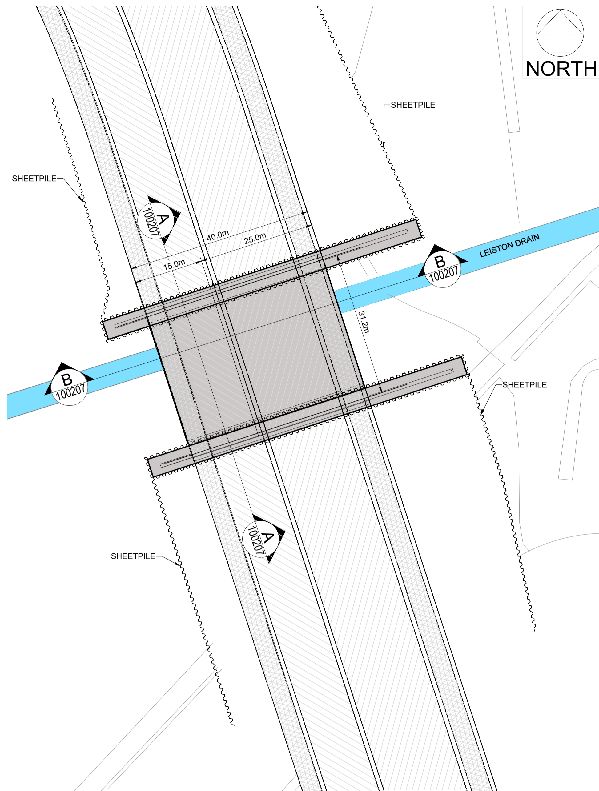
PLAN SCALE:1:500
